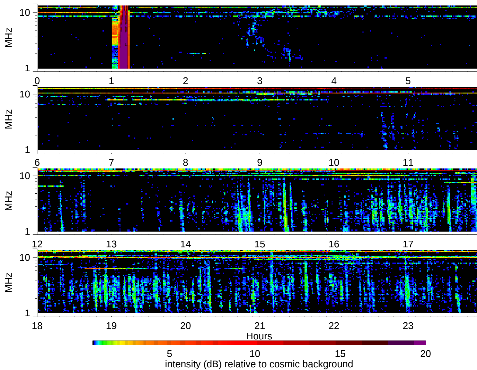
Wind Waves RAD2 receiver: 1998/6/27
