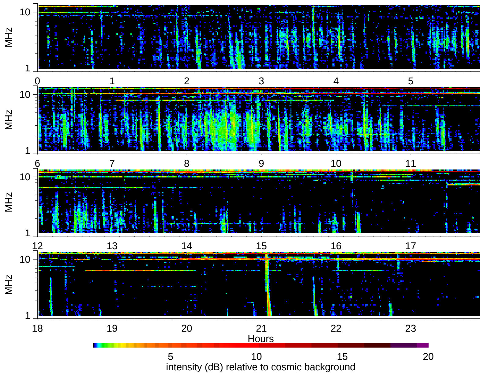
Wind Waves RAD2 receiver: 1998/6/28
