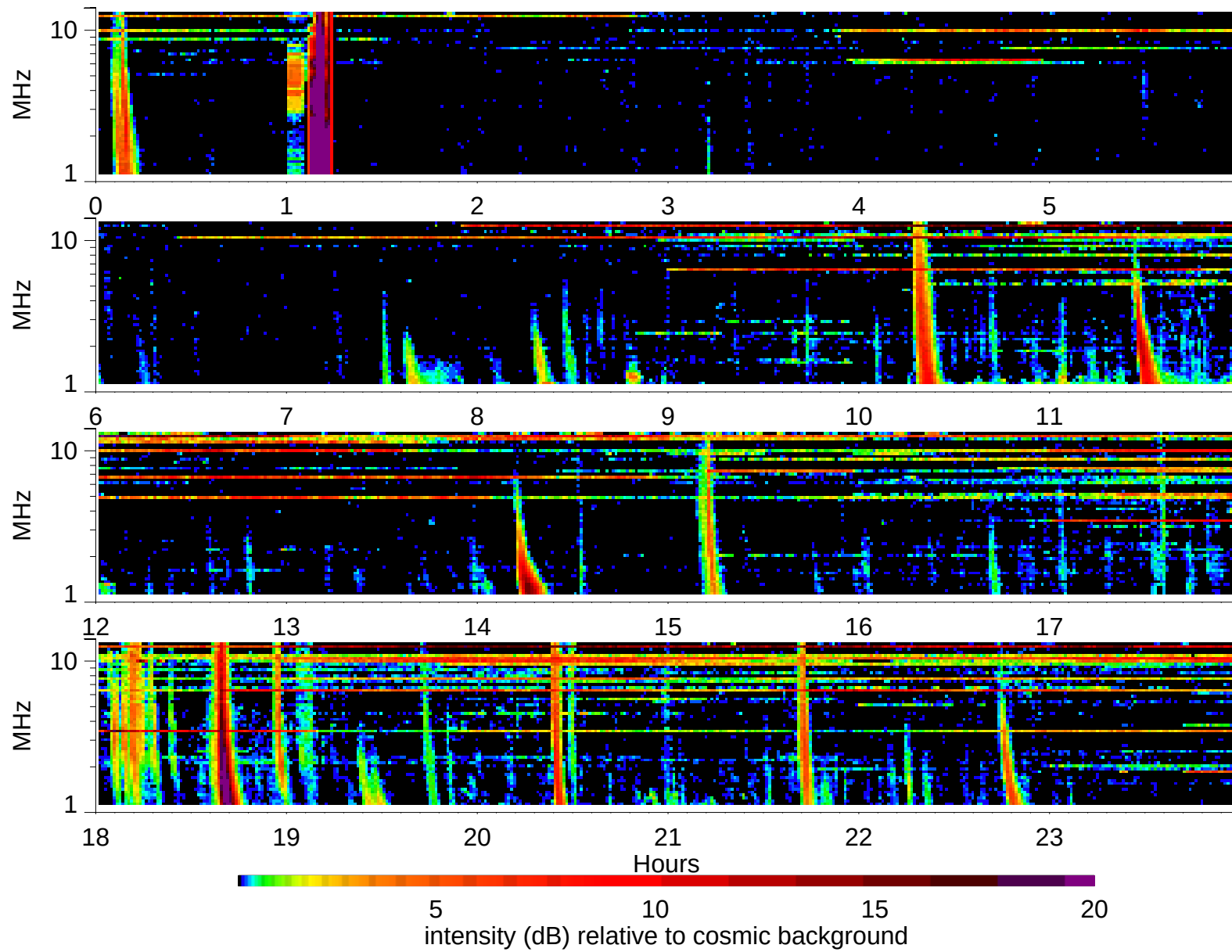
Wind Waves RAD2 receiver: 1998/7/1
