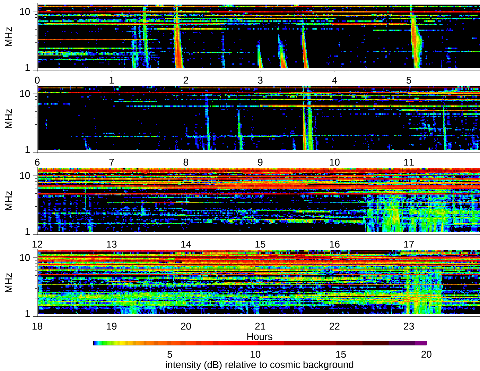
Wind Waves RAD2 receiver: 1998/7/2
