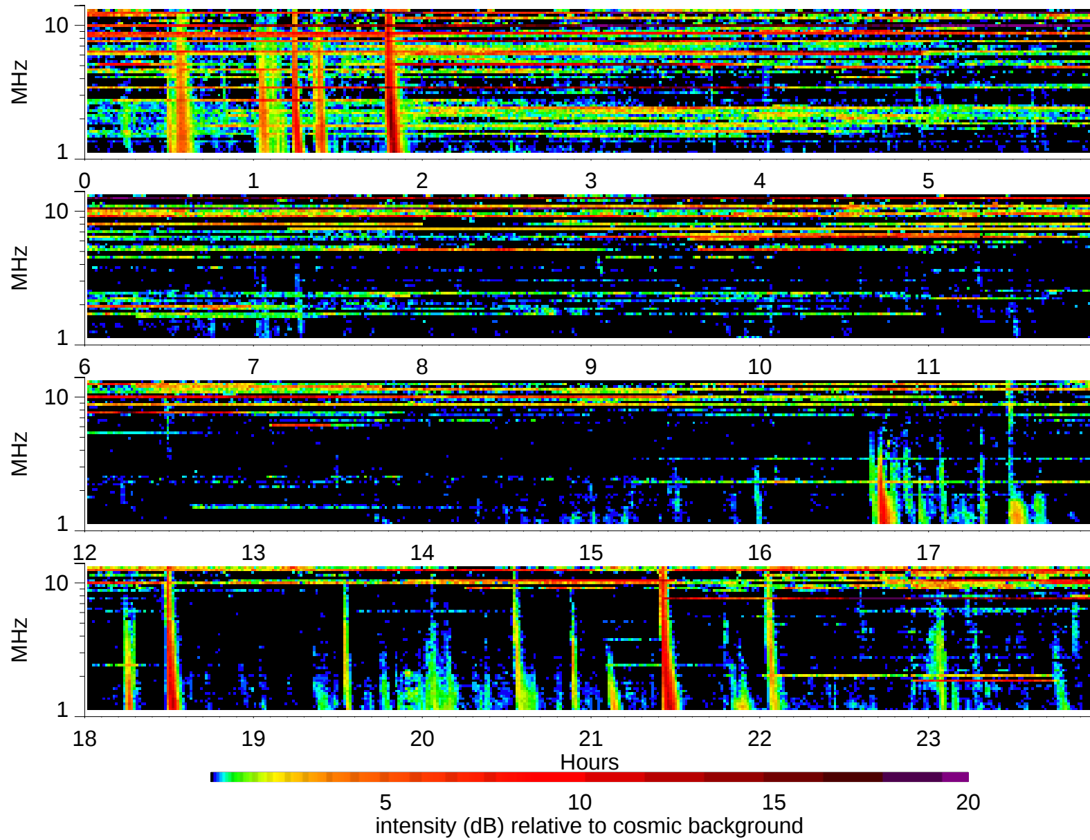
Wind Waves RAD2 receiver: 1998/7/3
