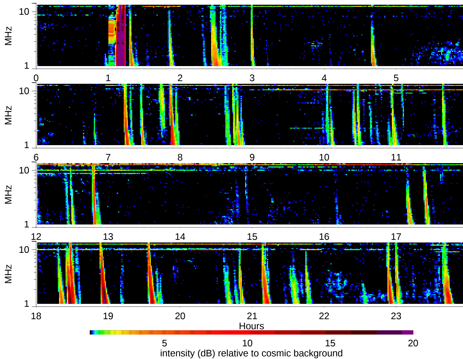
Wind Waves RAD2 receiver: 1998/7/11
