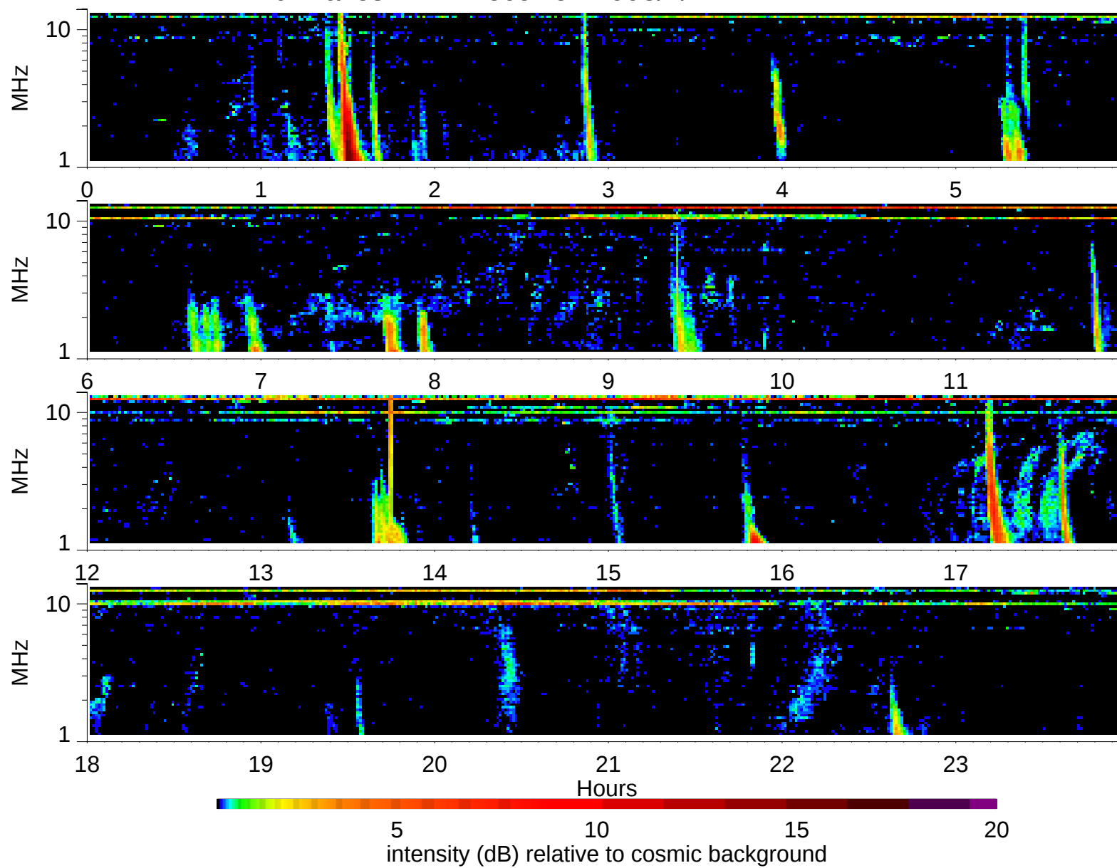
Wind Waves RAD2 receiver: 1998/7/12
