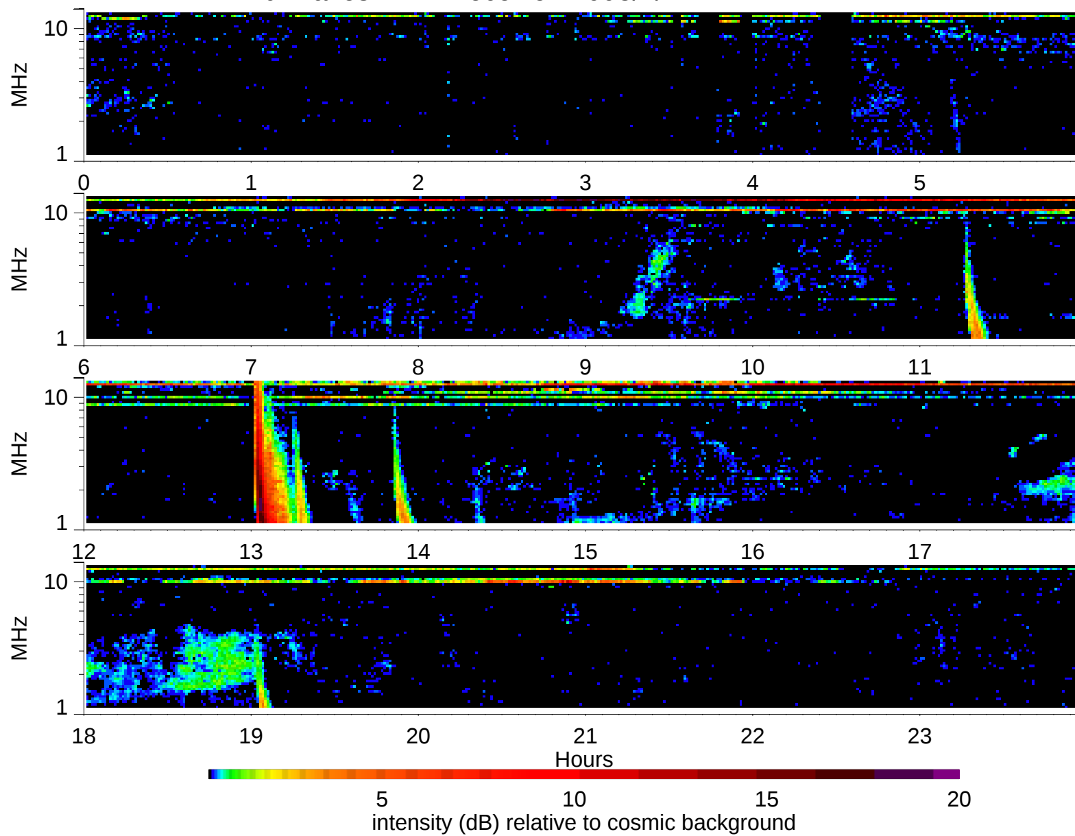
Wind Waves RAD2 receiver: 1998/7/14
