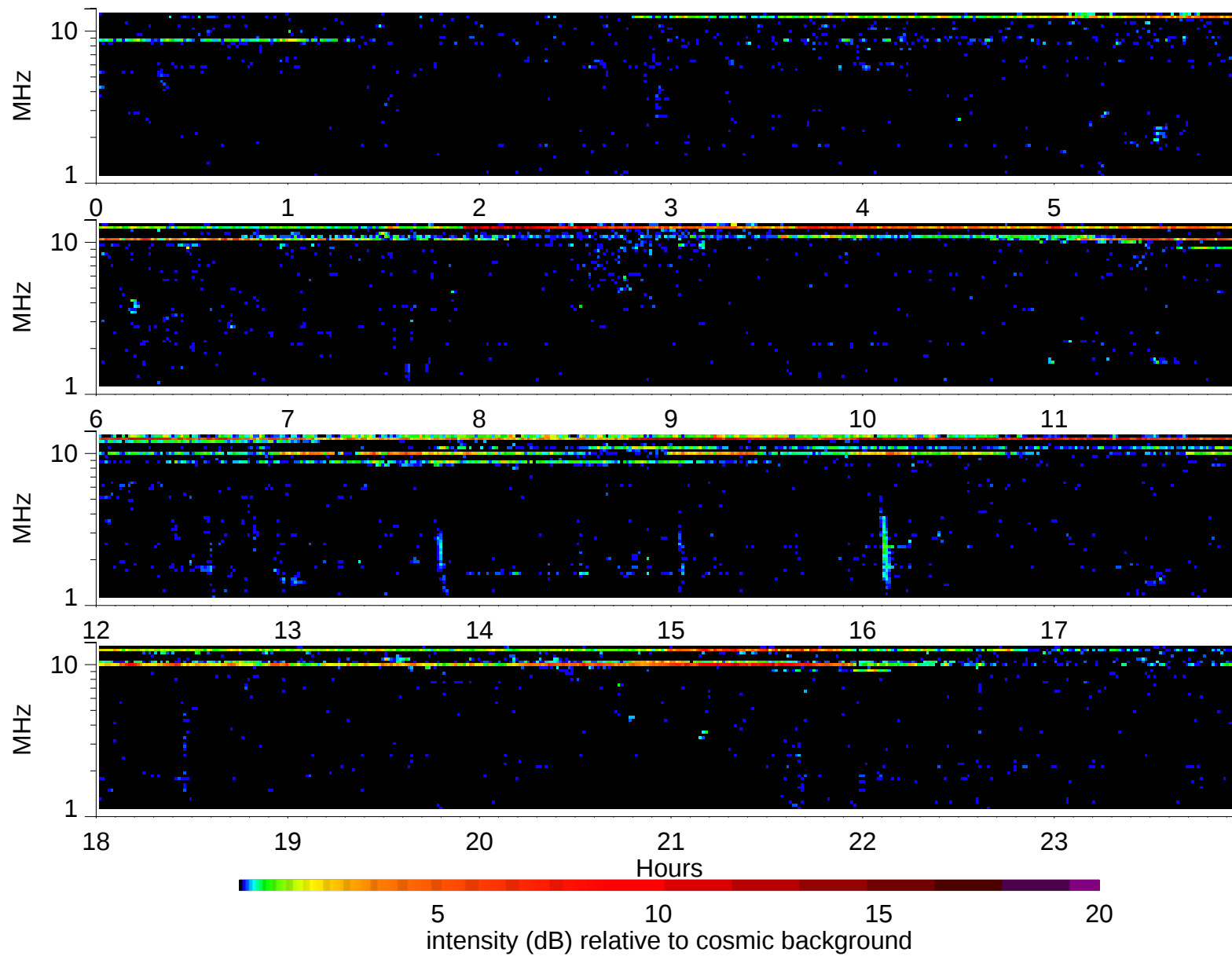
Wind Waves RAD2 receiver: 1998/7/18
