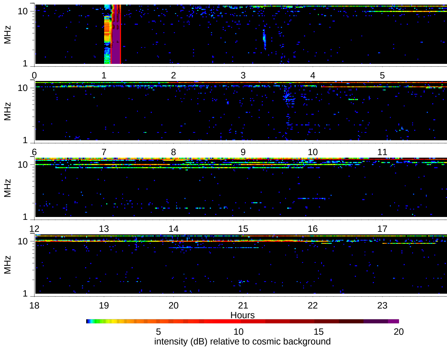
Wind Waves RAD2 receiver: 1998/7/19
