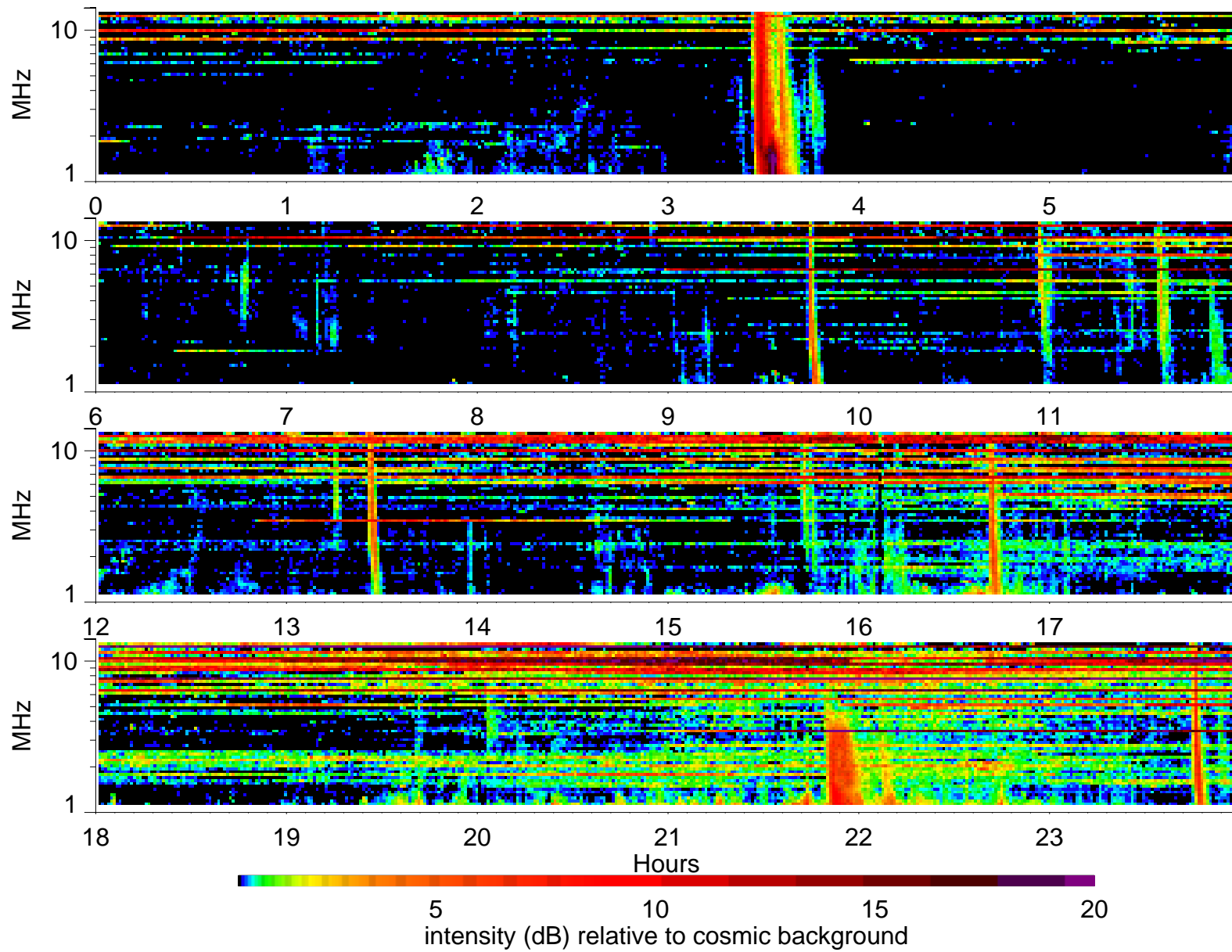
Wind Waves RAD2 receiver: 1998/7/24
