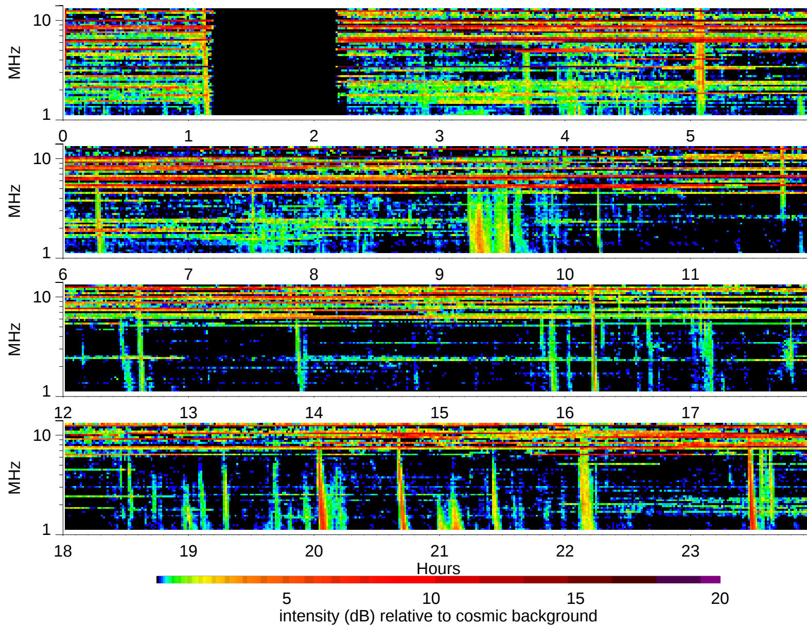
Wind Waves RAD2 receiver: 1998/7/25
