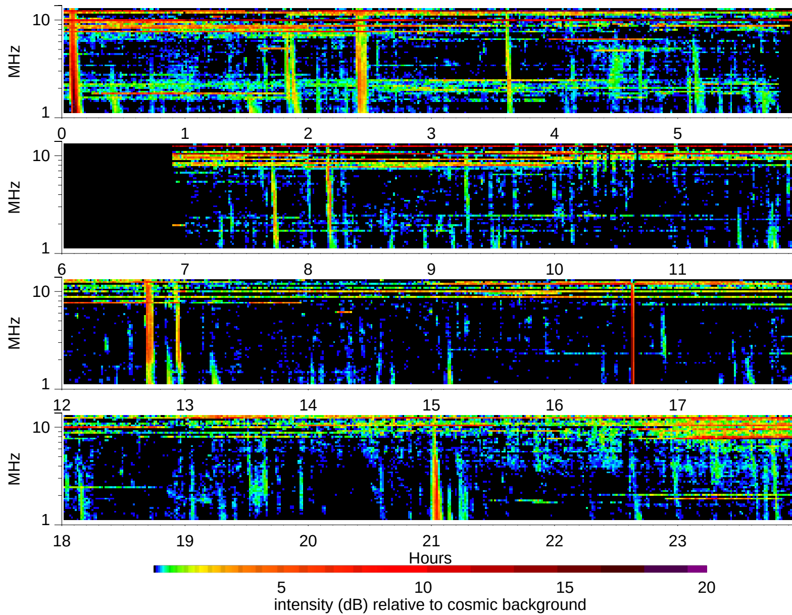
Wind Waves RAD2 receiver: 1998/7/26
