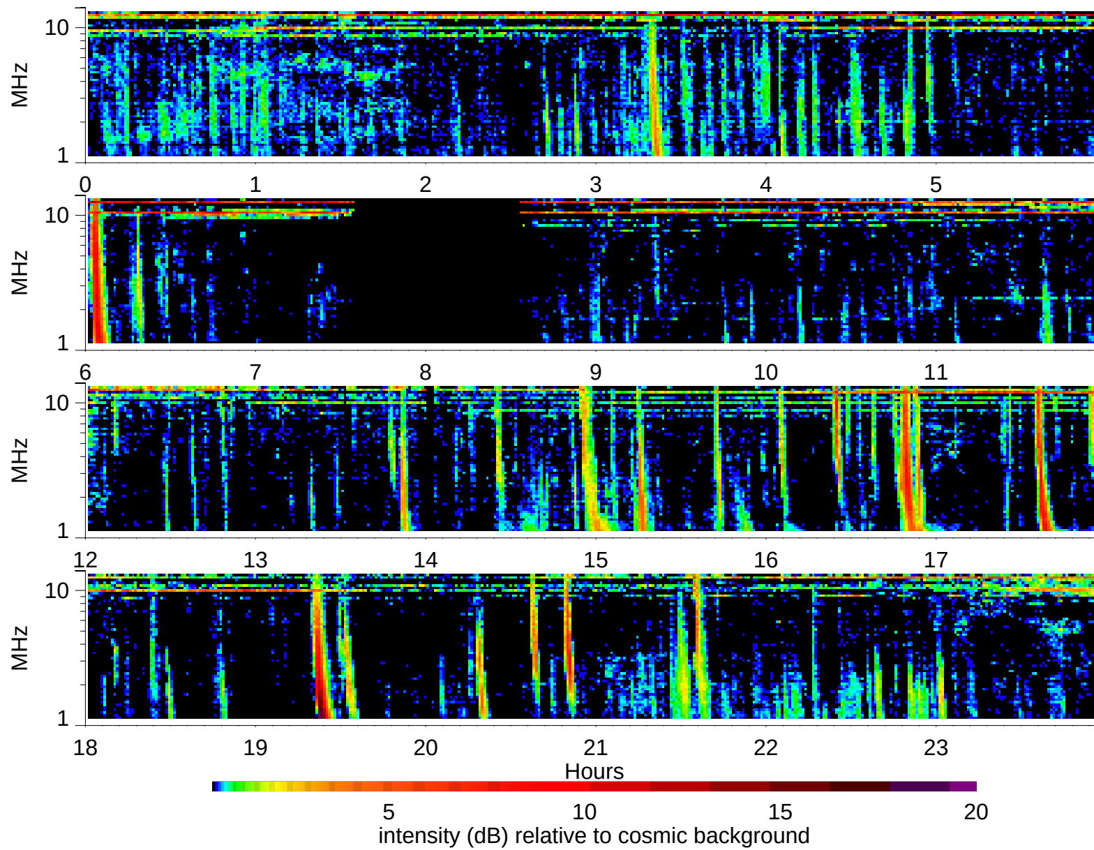
Wind Waves RAD2 receiver: 1998/7/28
