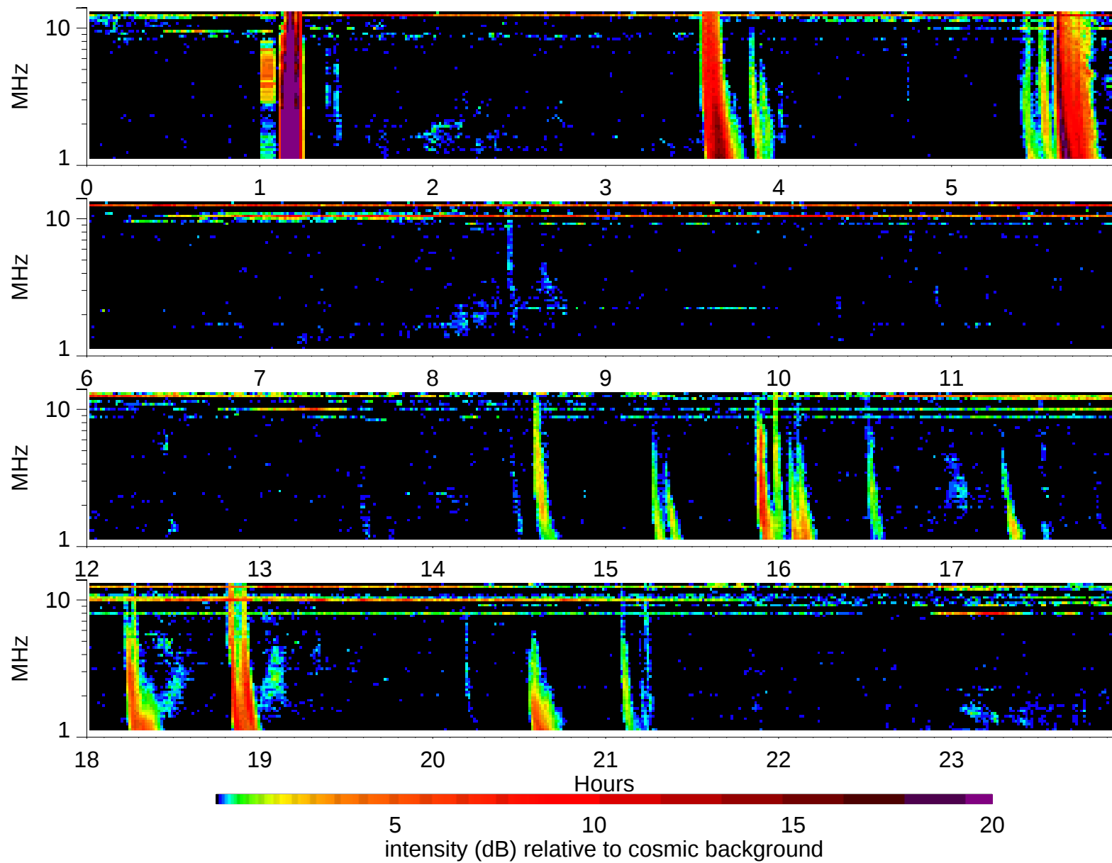
Wind Waves RAD2 receiver: 1998/7/31
