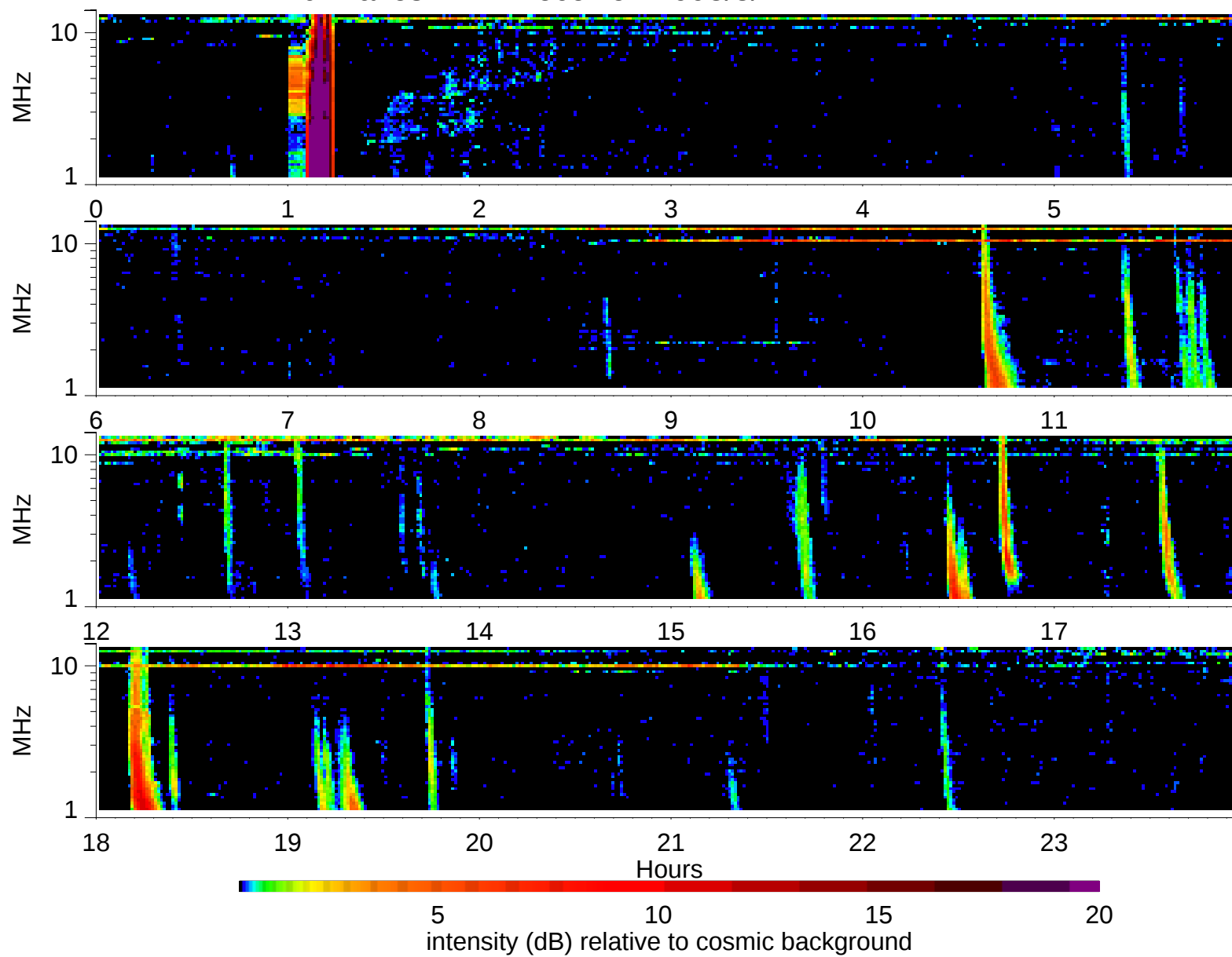
Wind Waves RAD2 receiver: 1998/8/4
