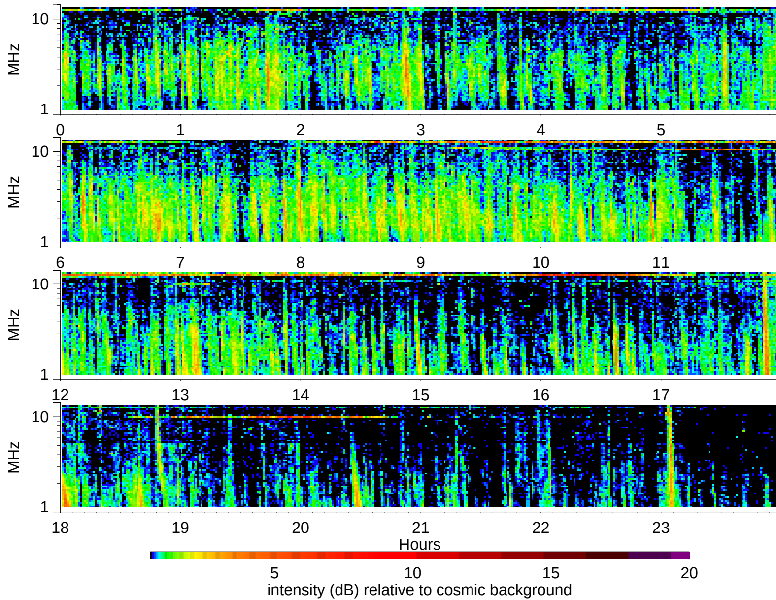
Wind Waves RAD2 receiver: 1998/8/9
