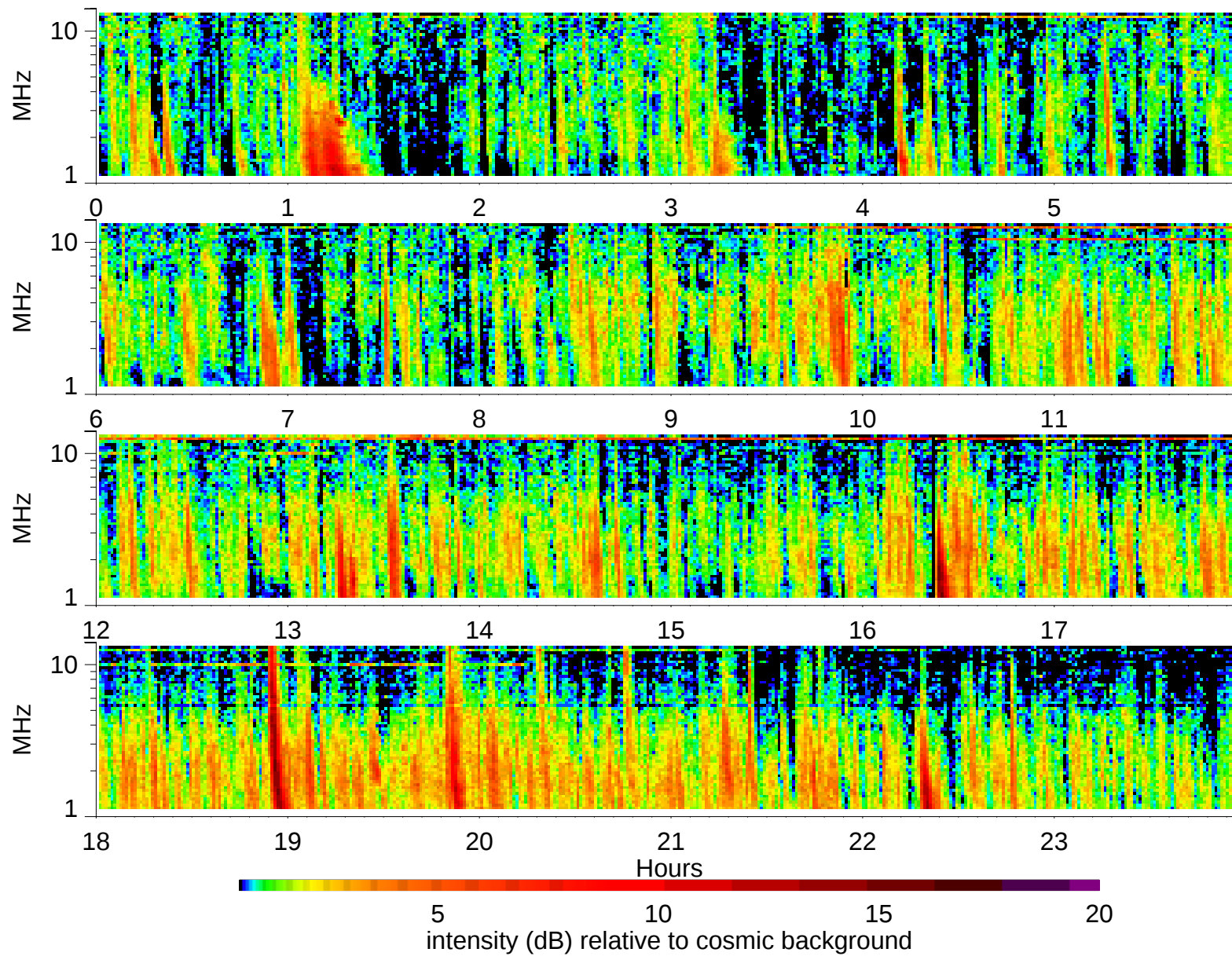
Wind Waves RAD2 receiver: 1998/8/11
