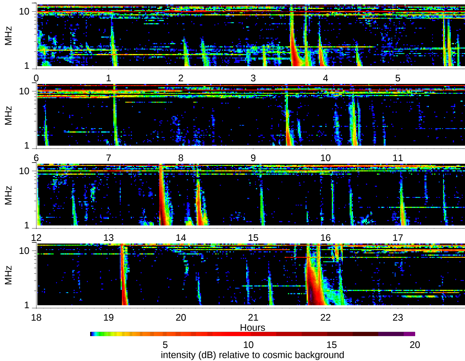
Wind Waves RAD2 receiver: 1998/8/19
