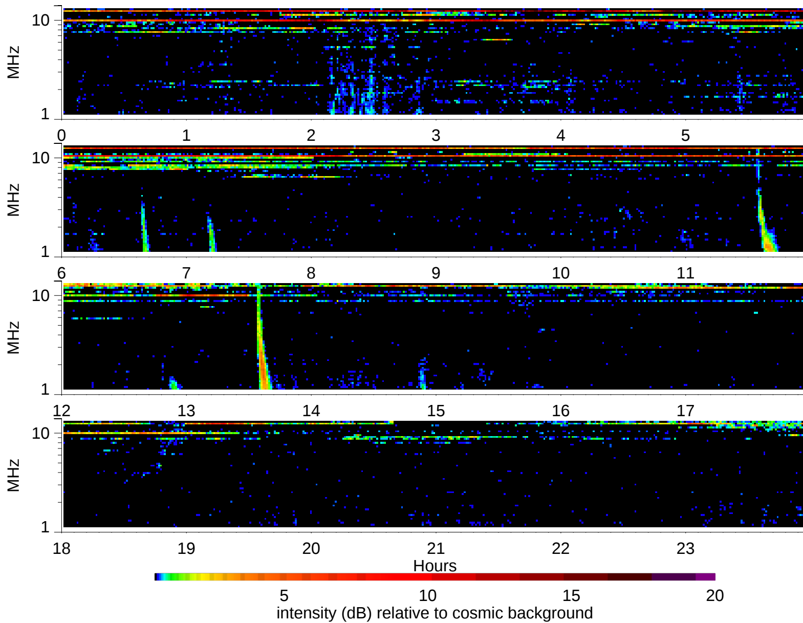
Wind Waves RAD2 receiver: 1998/8/21
