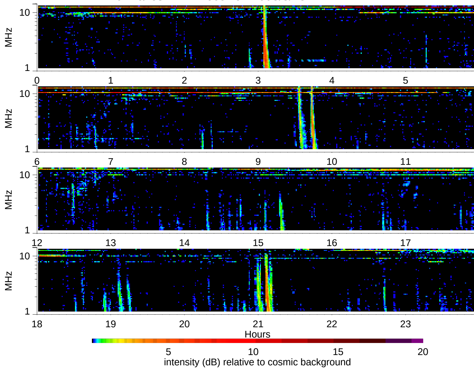
Wind Waves RAD2 receiver: 1998/8/23
