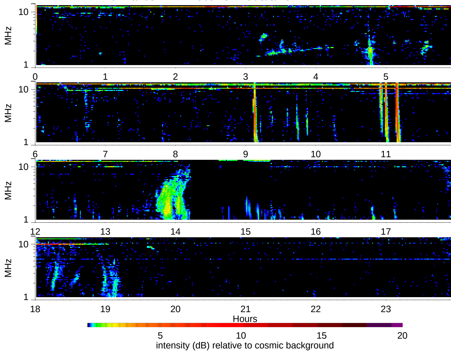
Wind Waves RAD2 receiver: 1998/8/25
