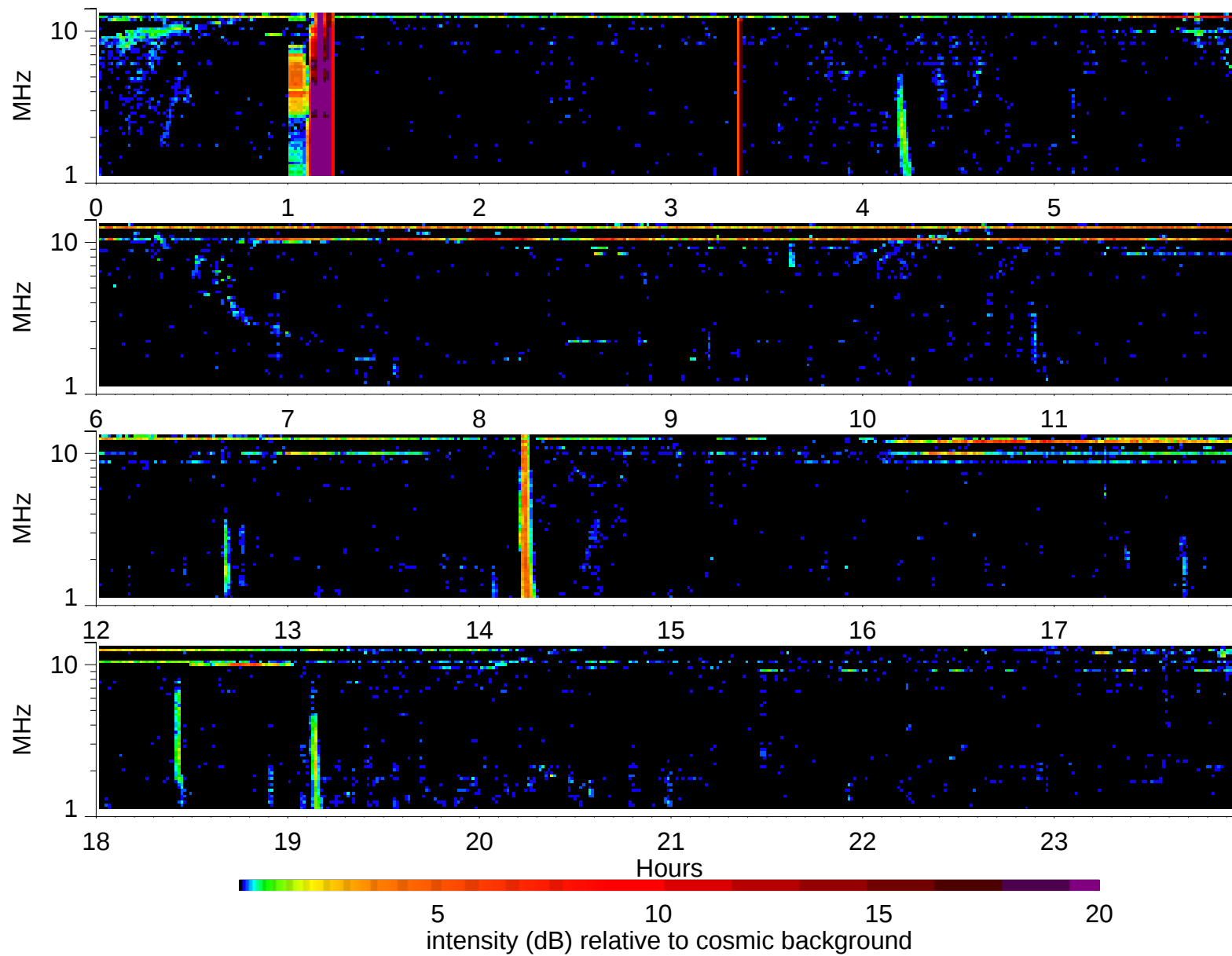
Wind Waves RAD2 receiver: 1998/8/26
