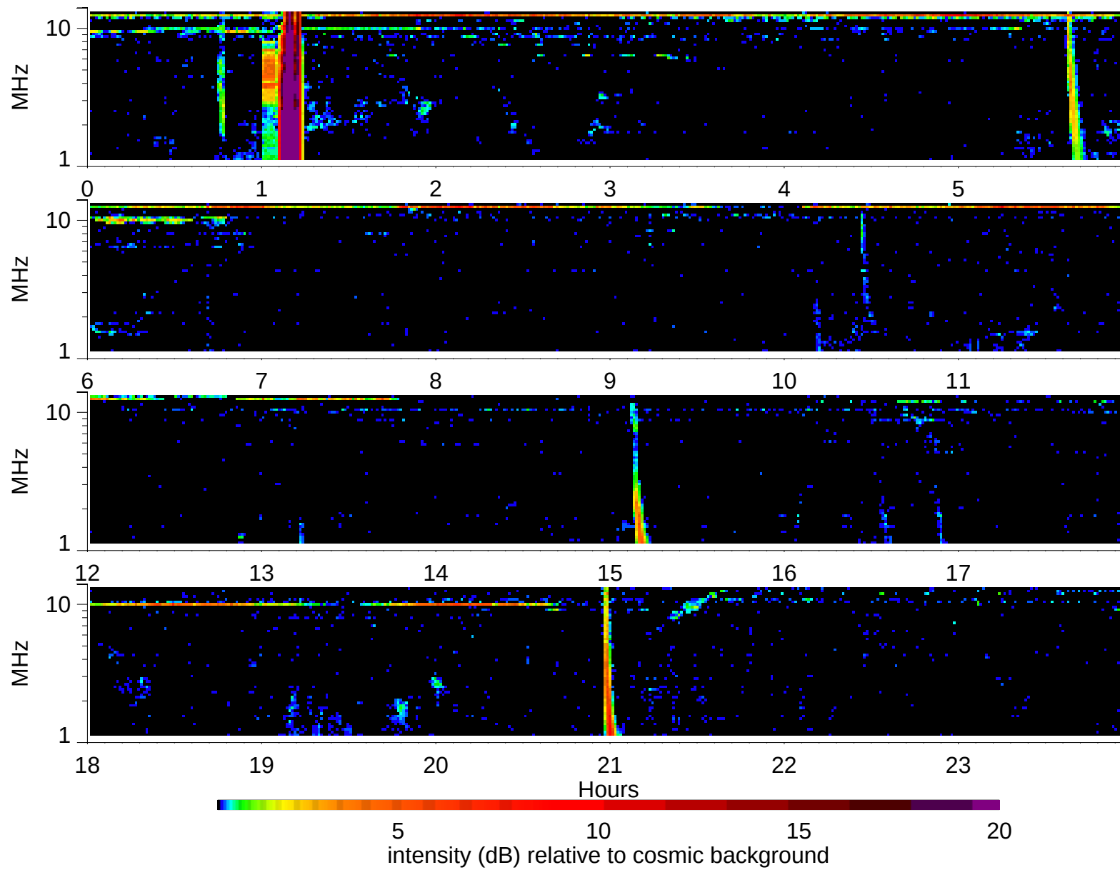
Wind Waves RAD2 receiver: 1998/8/28
