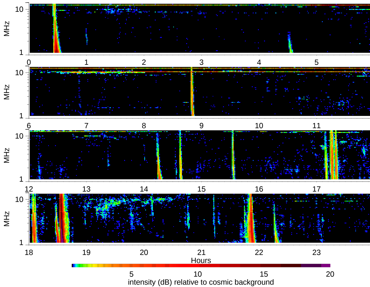
Wind Waves RAD2 receiver: 1998/8/29
