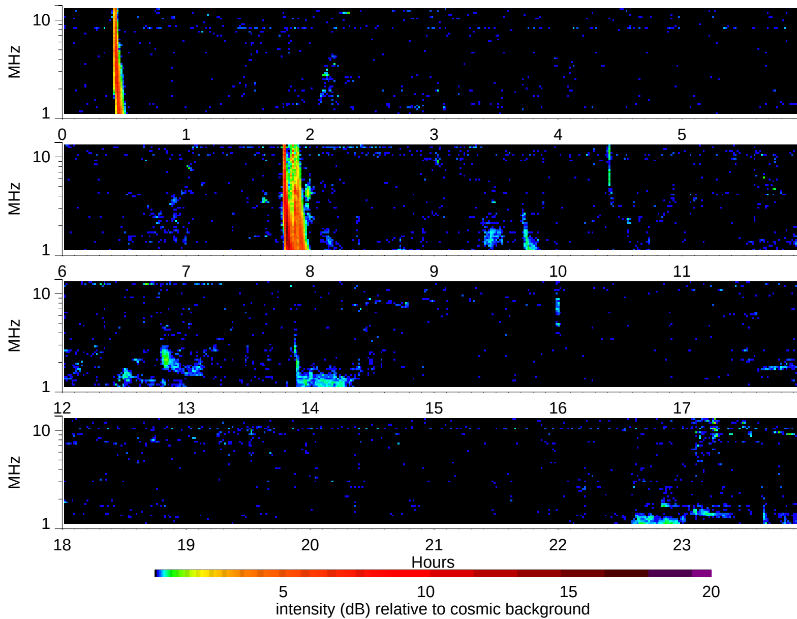
Wind Waves RAD2 receiver: 1998/9/12
