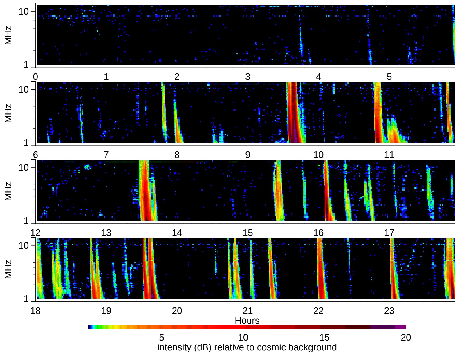
Wind Waves RAD2 receiver: 1998/9/14
