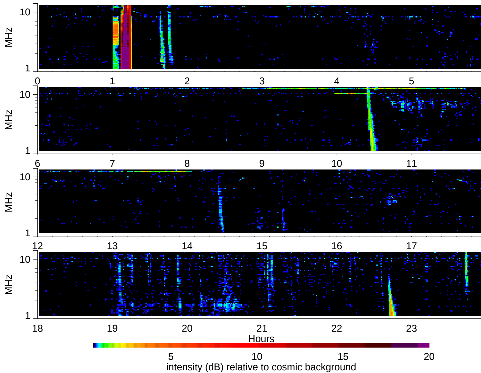
Wind Waves RAD2 receiver: 1998/9/15
