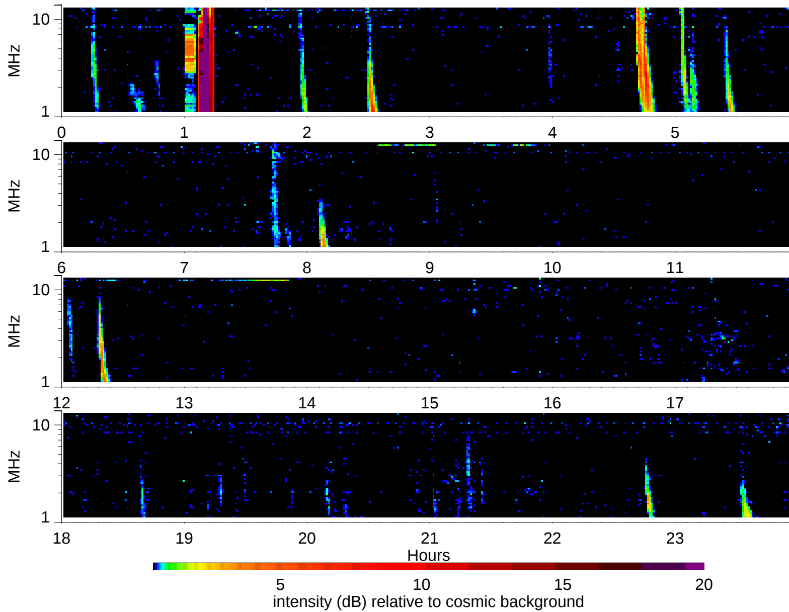
Wind Waves RAD2 receiver: 1998/9/17
