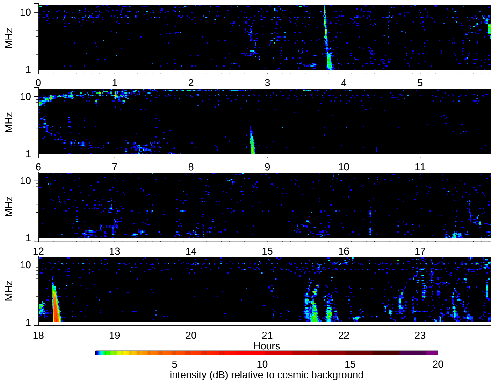
Wind Waves RAD2 receiver: 1998/9/18
