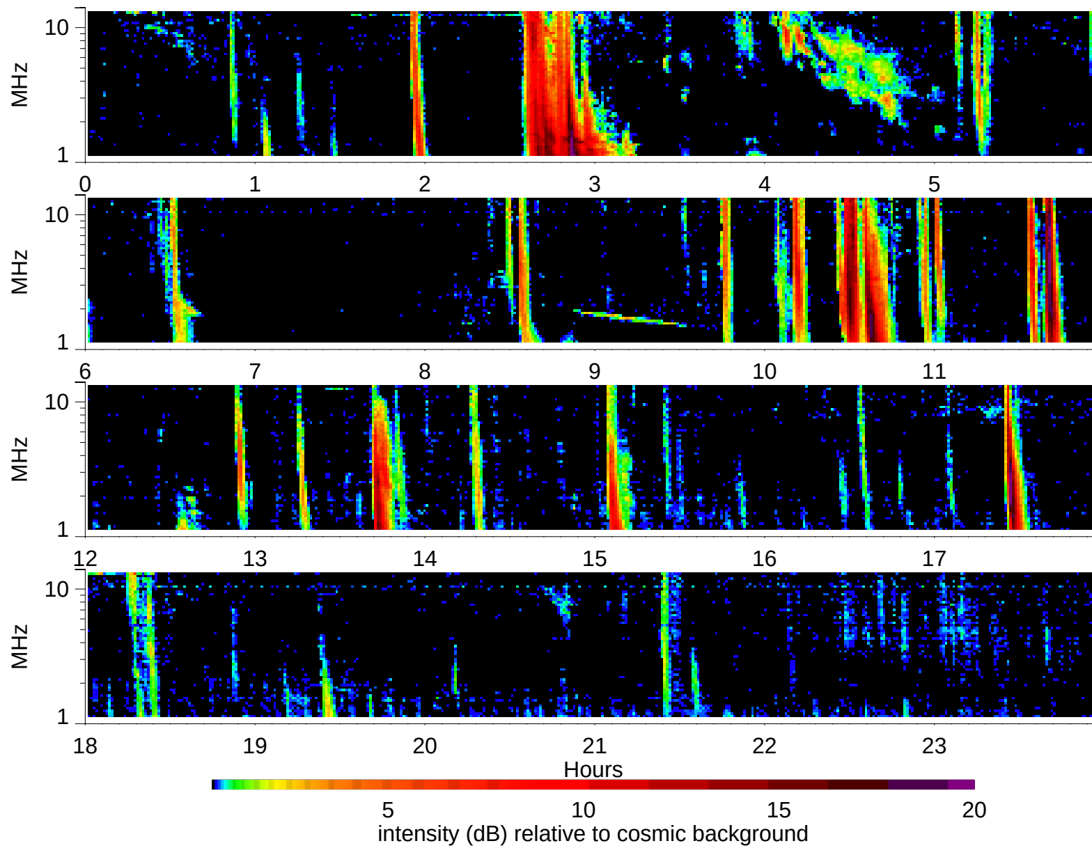
Wind Waves RAD2 receiver: 1998/9/20
