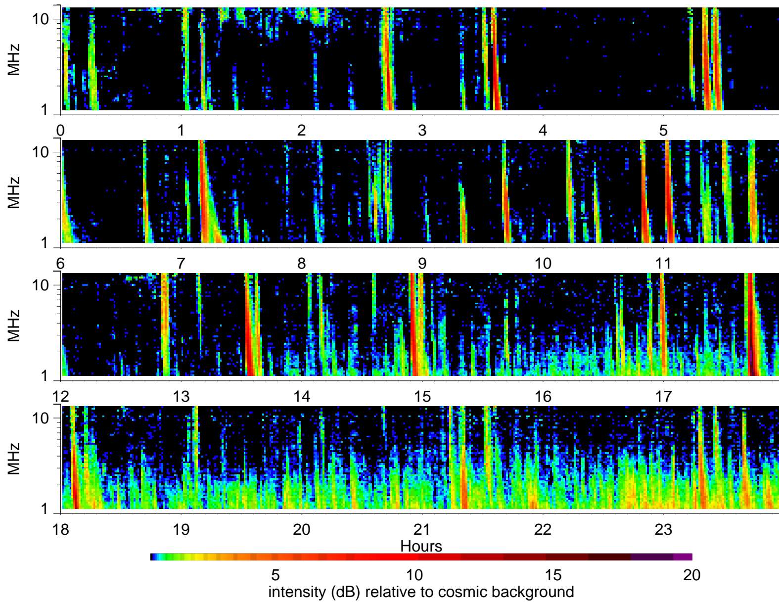
Wind Waves RAD2 receiver: 1998/9/22
