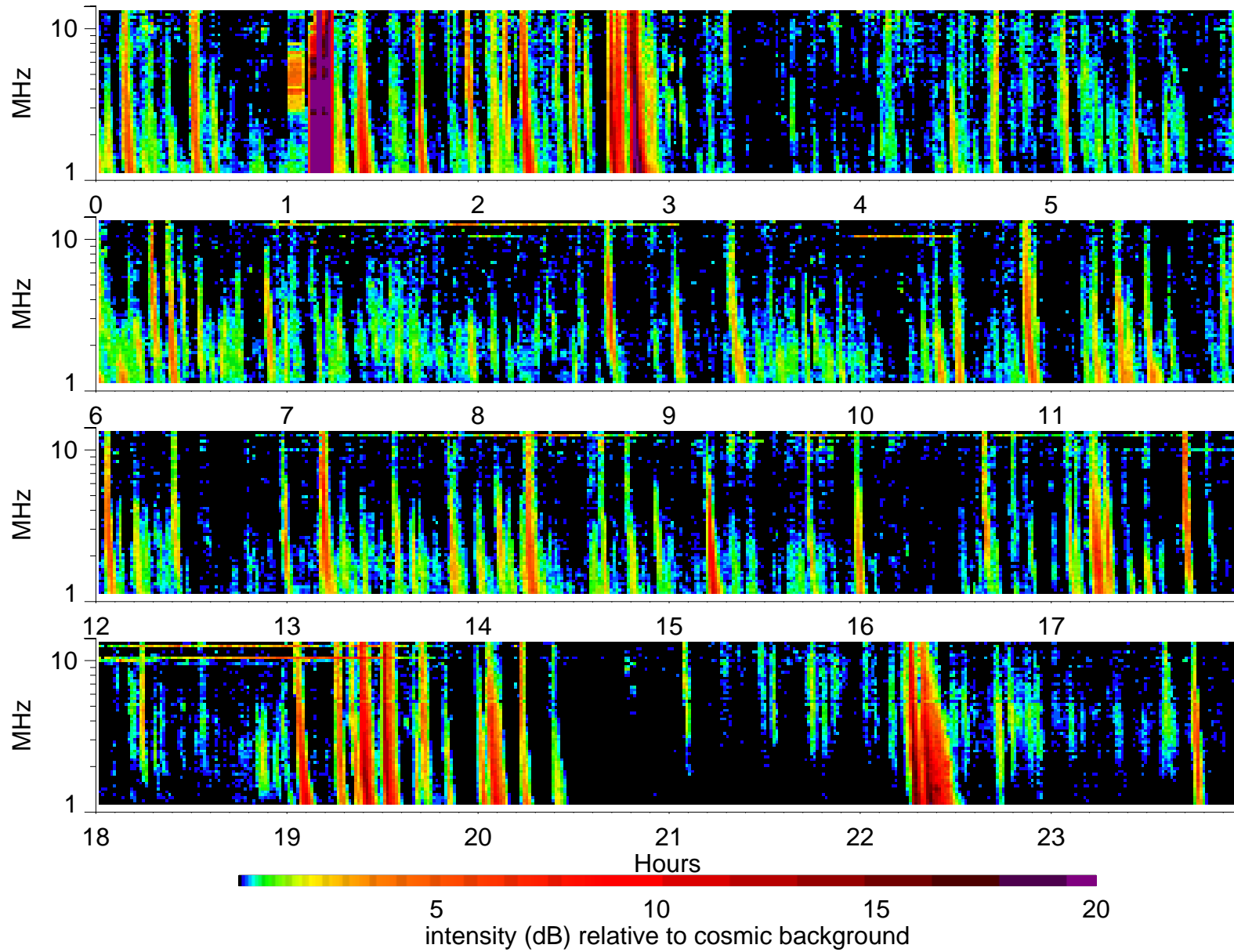
Wind Waves RAD2 receiver: 1998/9/25
