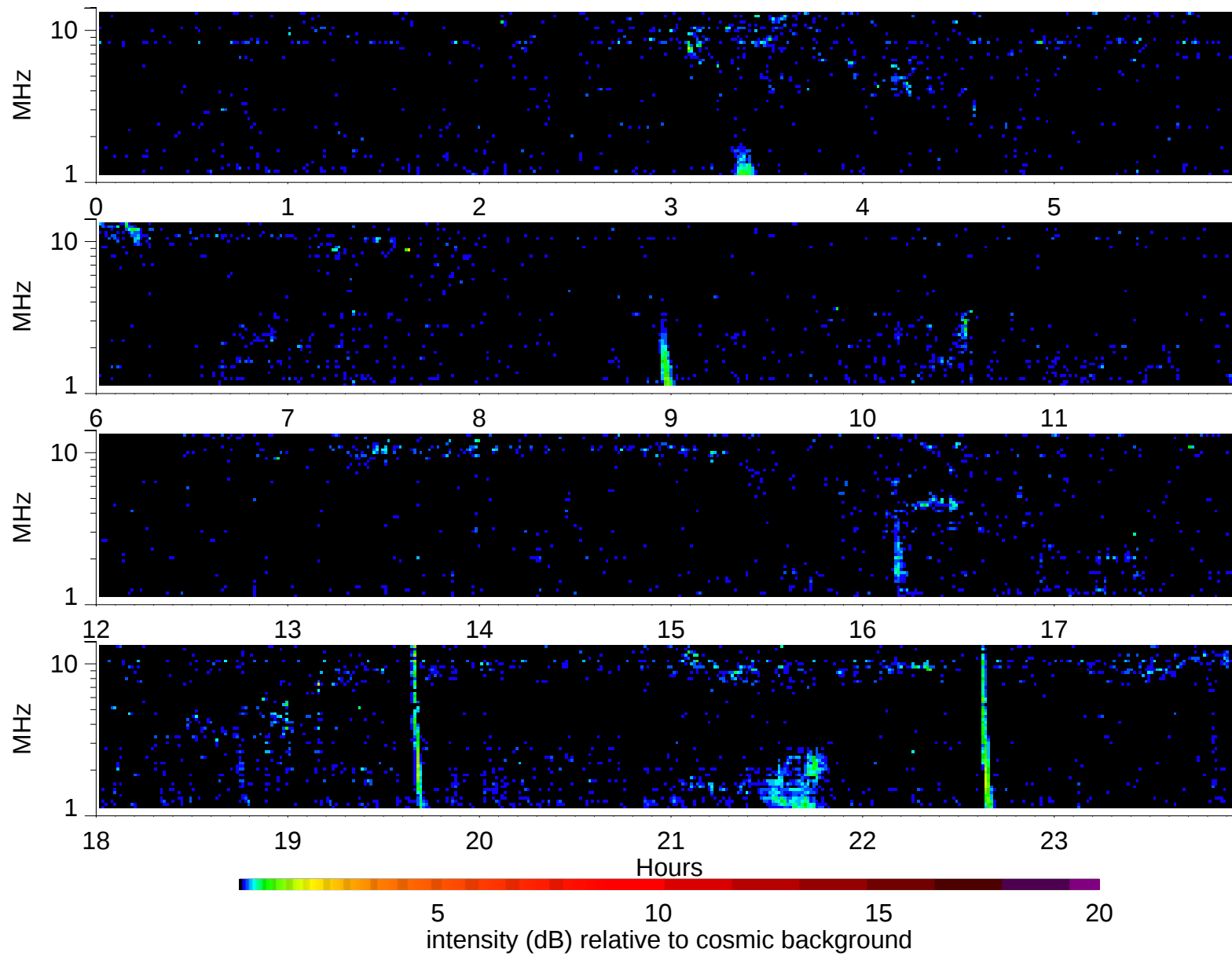
Wind Waves RAD2 receiver: 1998/10/4
