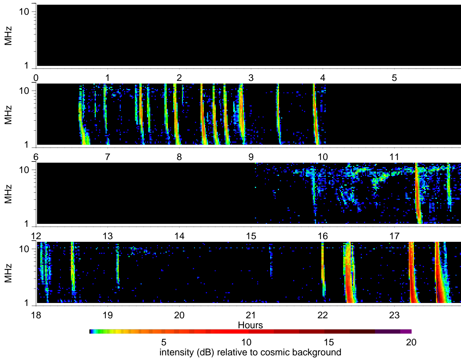
Wind Waves RAD2 receiver: 1998/10/7
