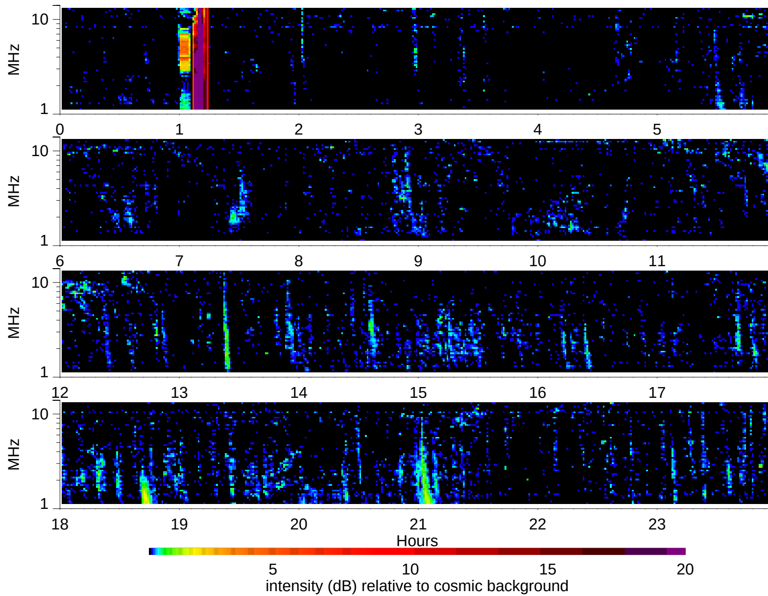
Wind Waves RAD2 receiver: 1998/10/9
