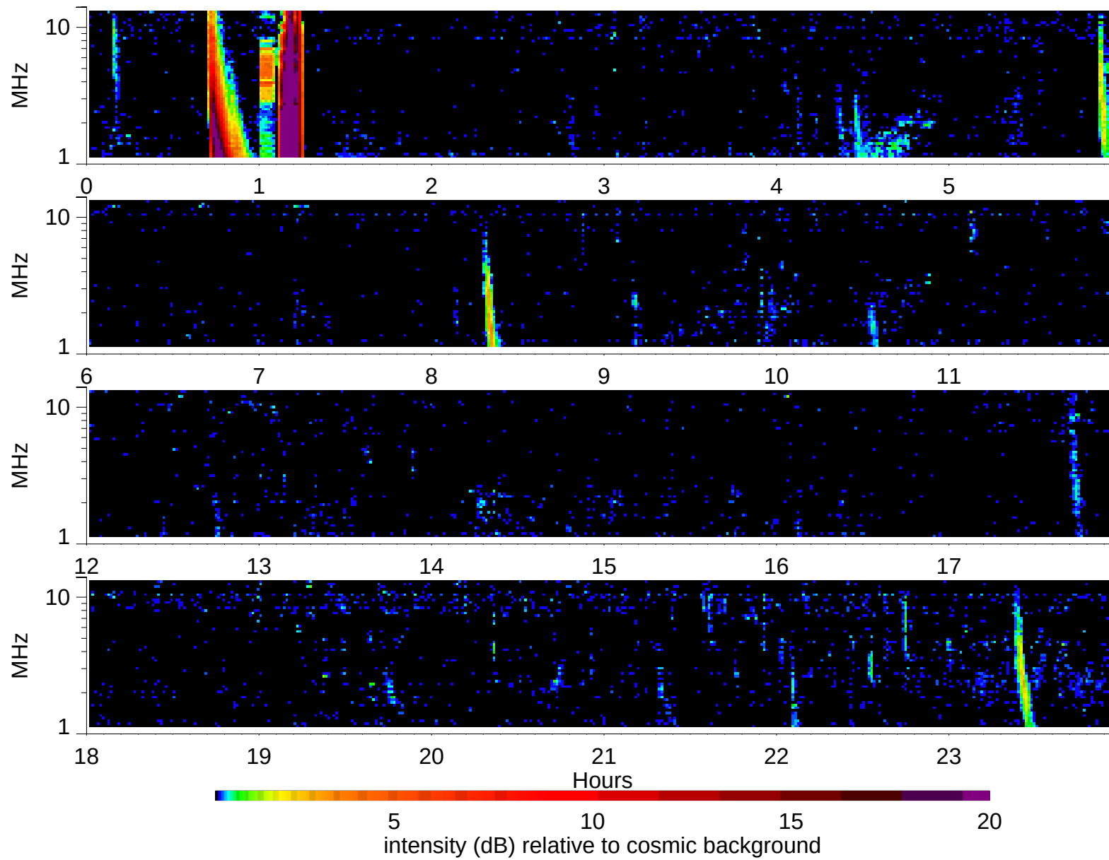
Wind Waves RAD2 receiver: 1998/10/15
