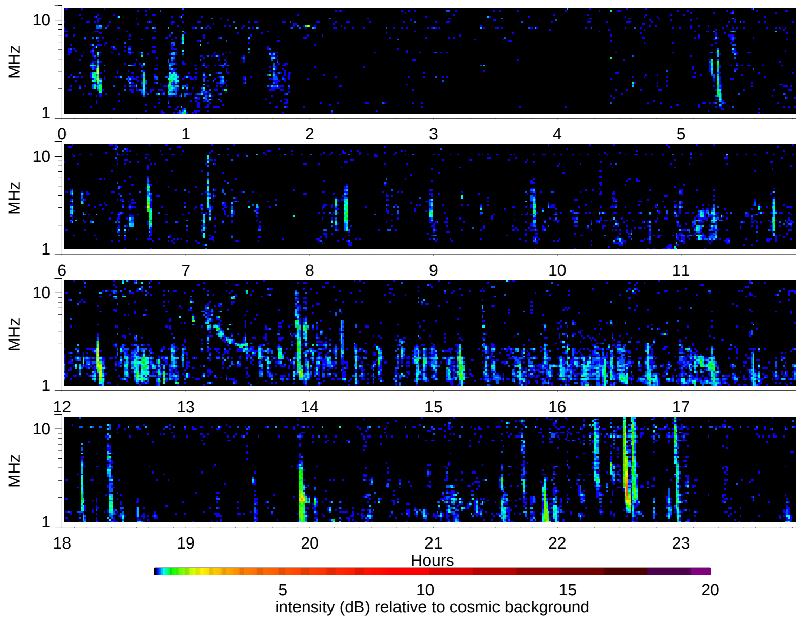
Wind Waves RAD2 receiver: 1998/10/16
