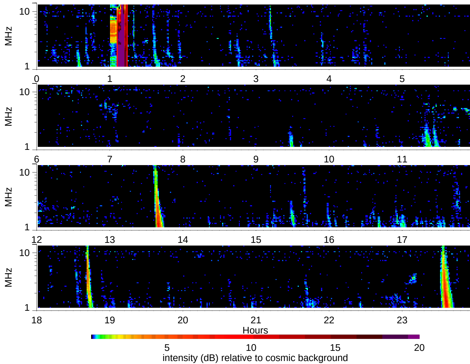
Wind Waves RAD2 receiver: 1998/10/17
