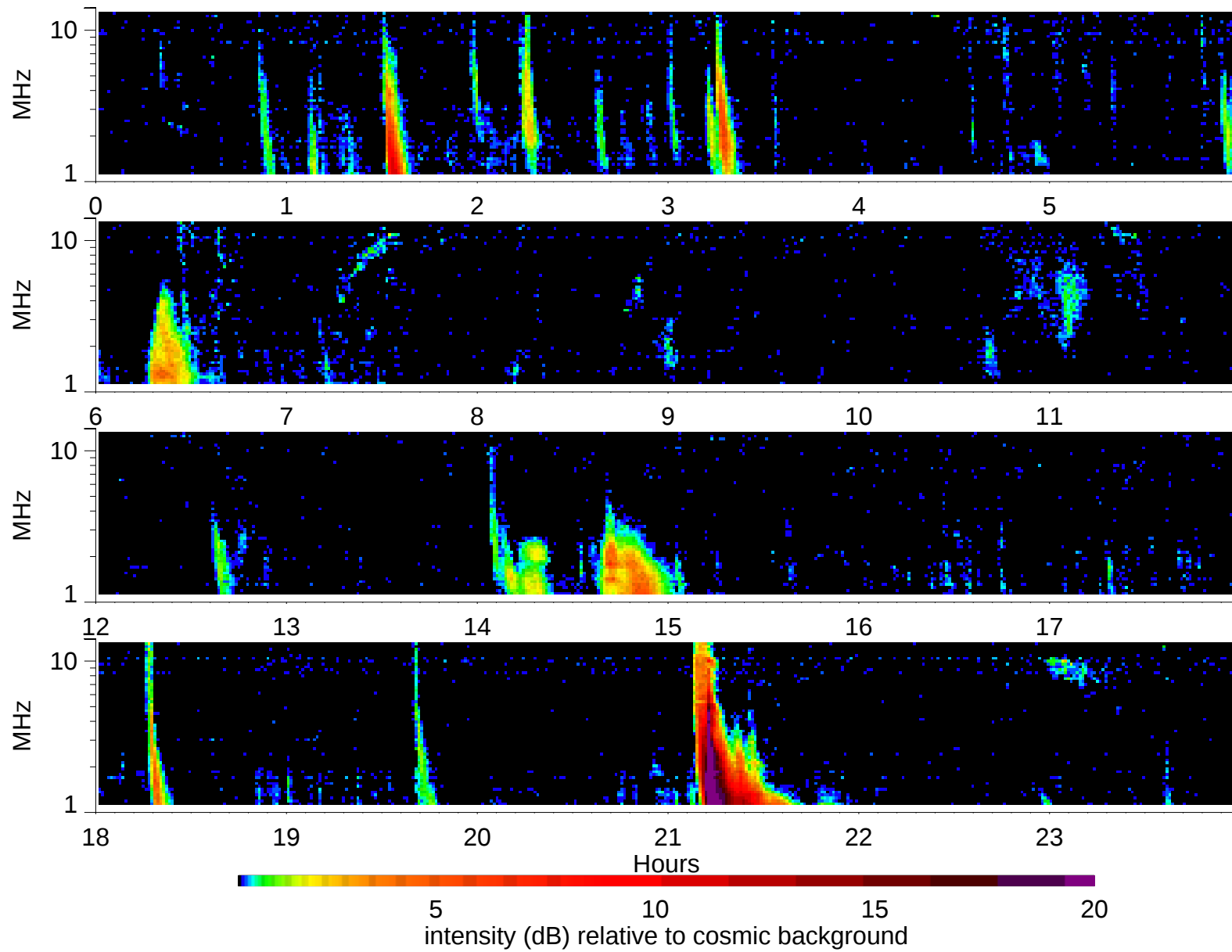
Wind Waves RAD2 receiver: 1998/10/18
