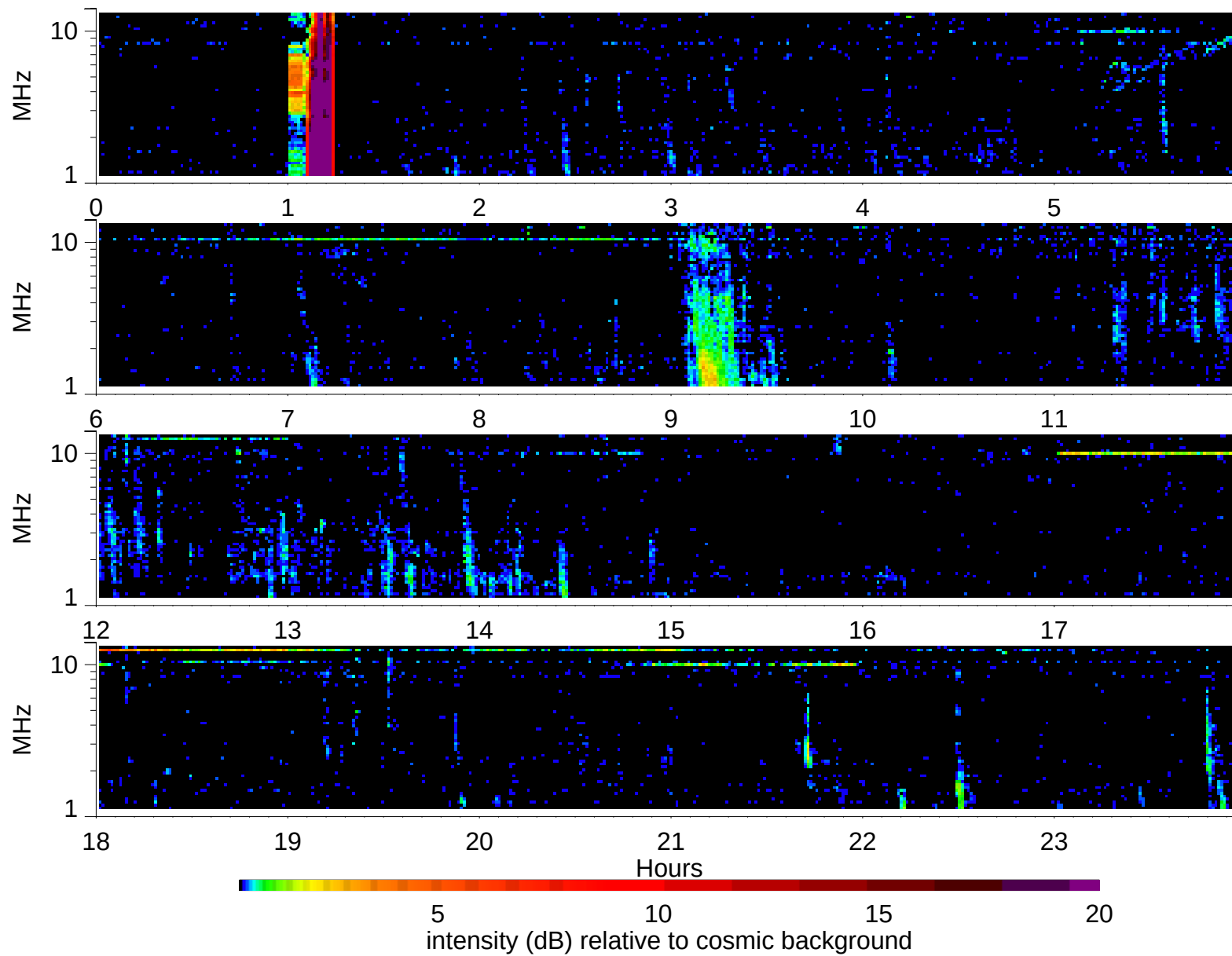
Wind Waves RAD2 receiver: 1998/10/19
