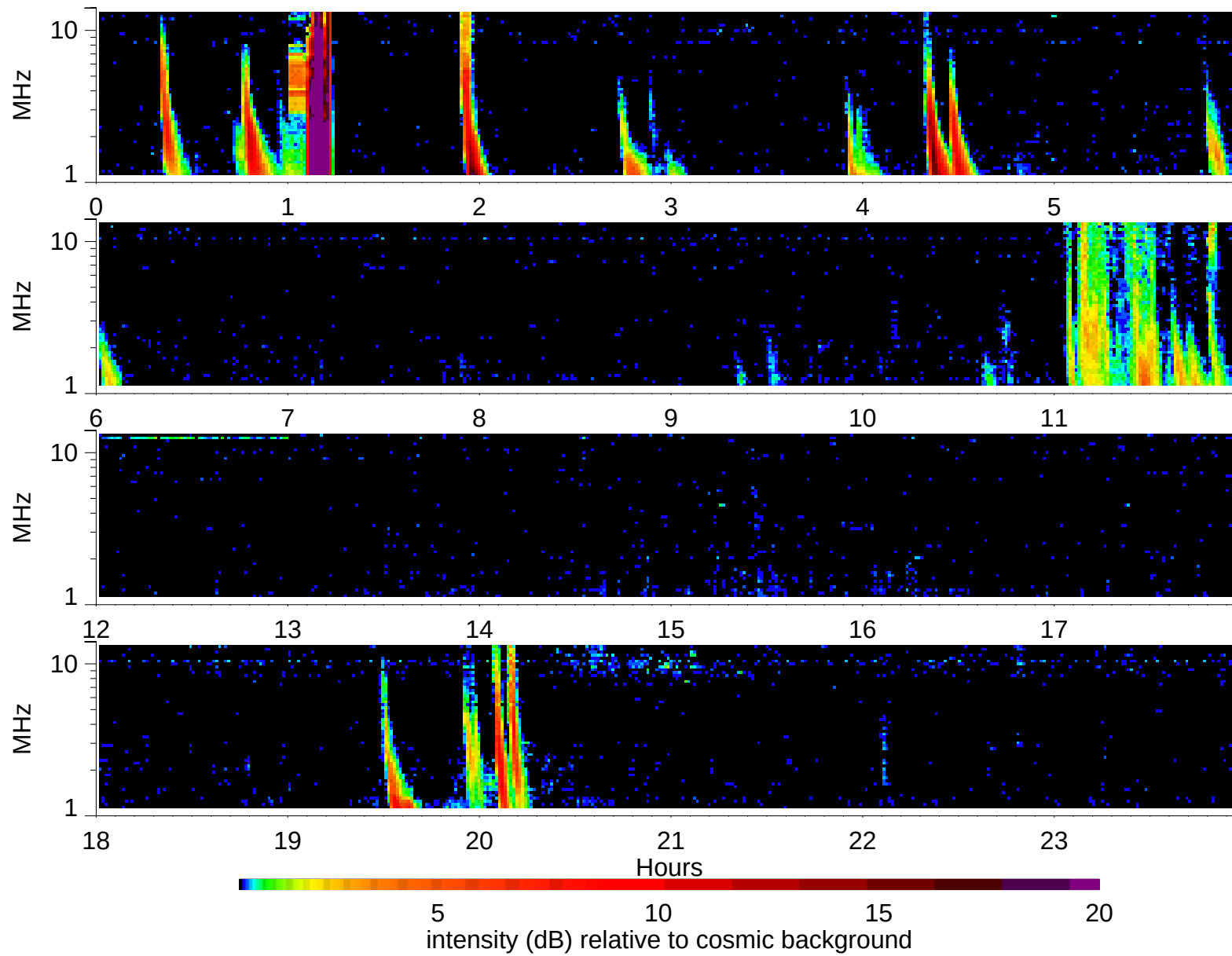
Wind Waves RAD2 receiver: 1998/10/21
