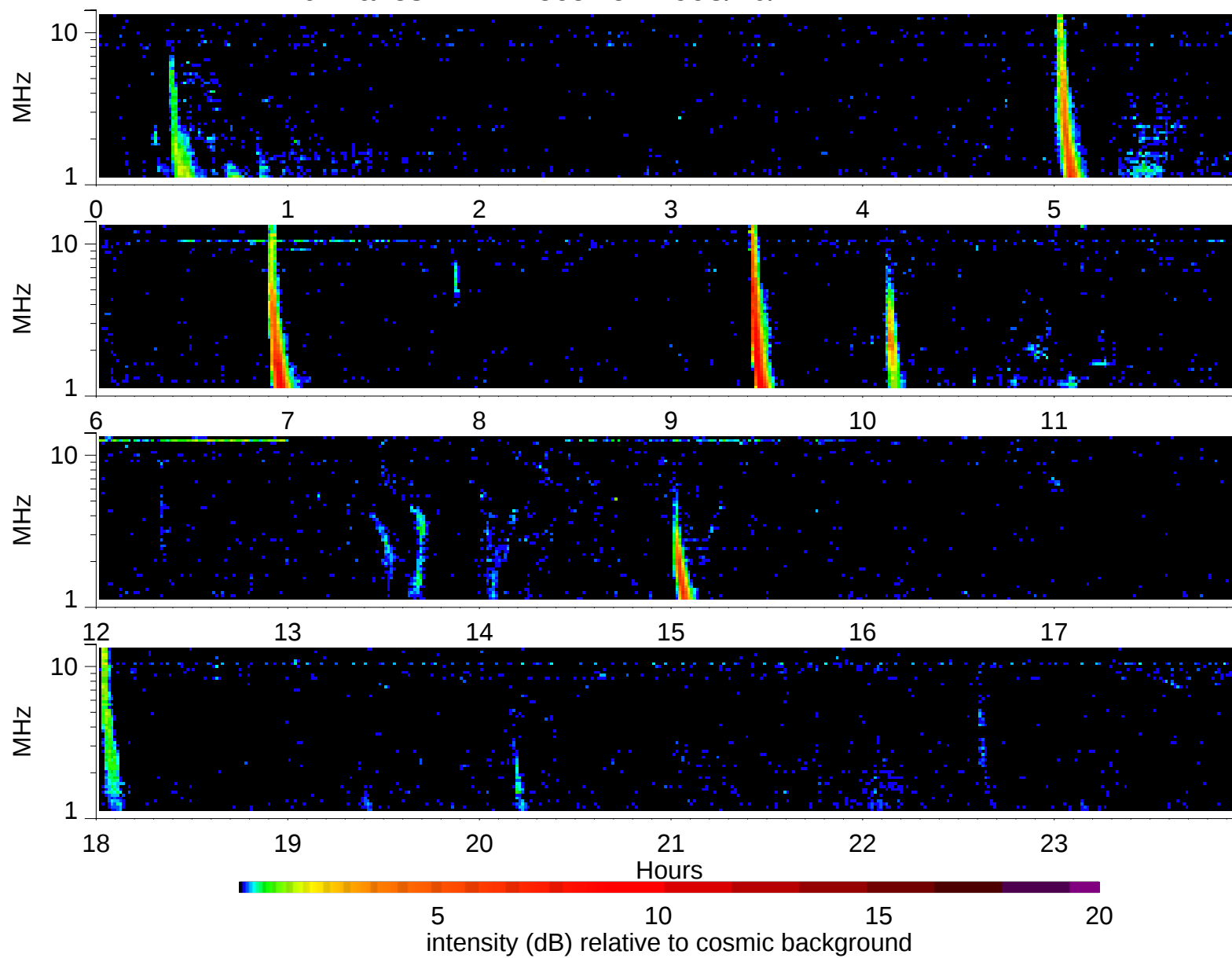
Wind Waves RAD2 receiver: 1998/10/22
