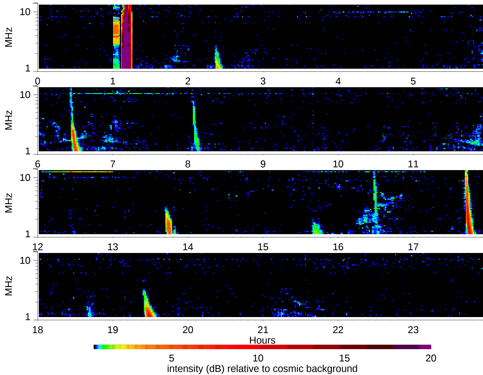
Wind Waves RAD2 receiver: 1998/10/23
