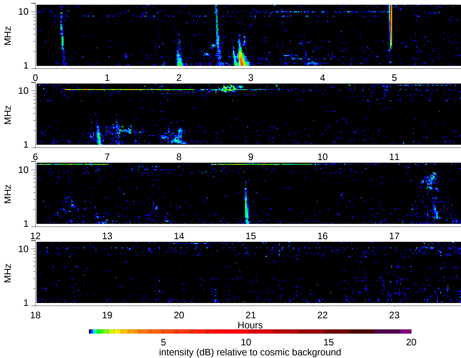
Wind Waves RAD2 receiver: 1998/10/24
