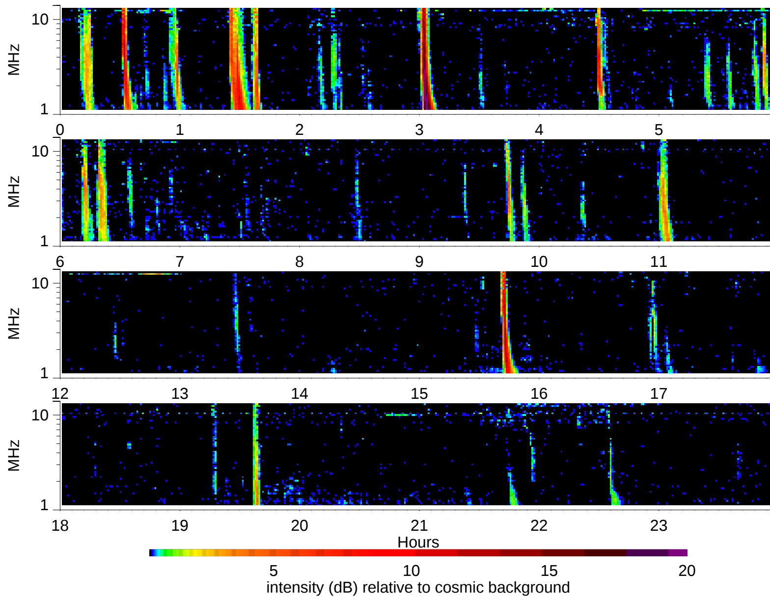
Wind Waves RAD2 receiver: 1998/10/28
