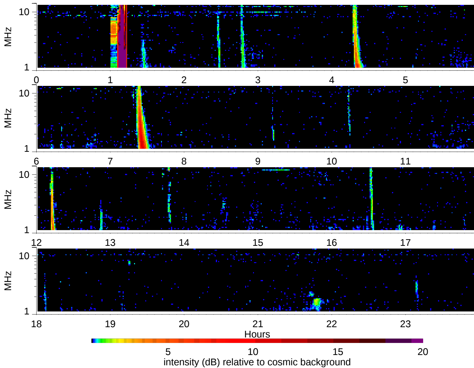
Wind Waves RAD2 receiver: 1998/10/29
