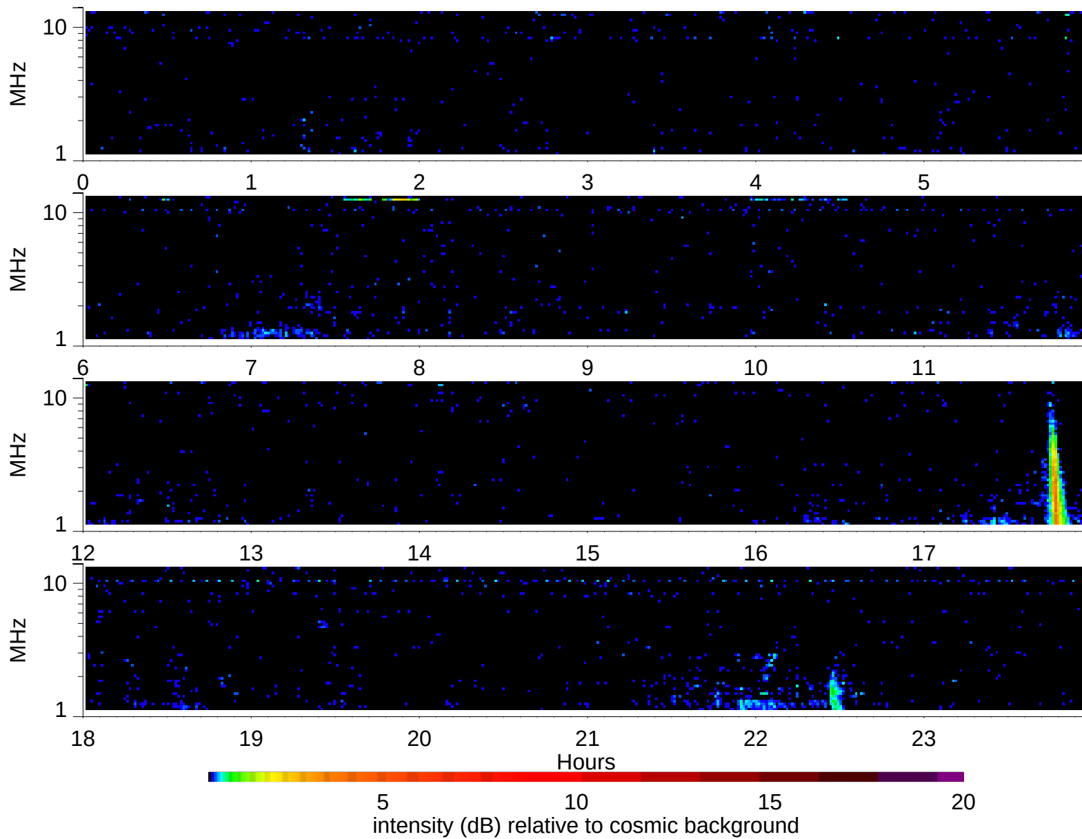
Wind Waves RAD2 receiver: 1998/10/30
