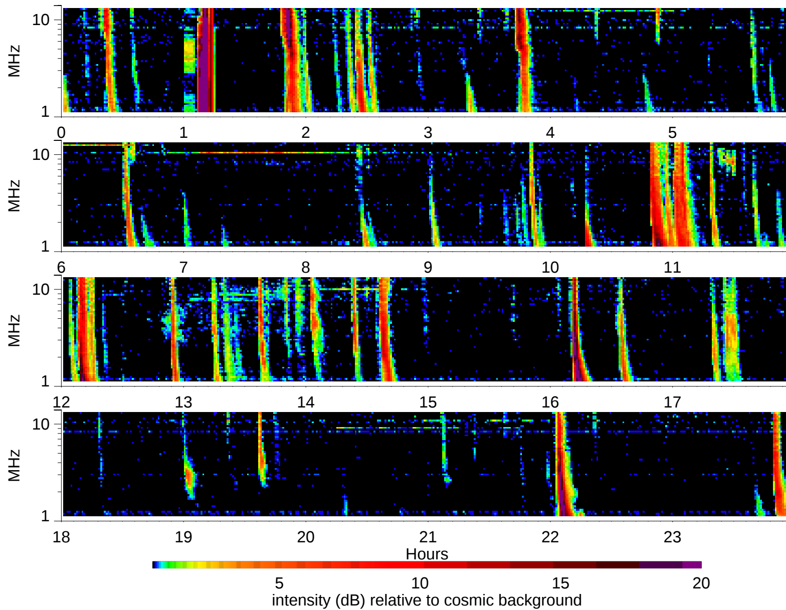
Wind Waves RAD2 receiver: 1998/11/8
