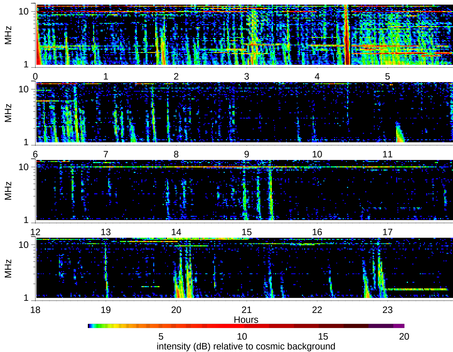
Wind Waves RAD2 receiver: 1998/11/15
